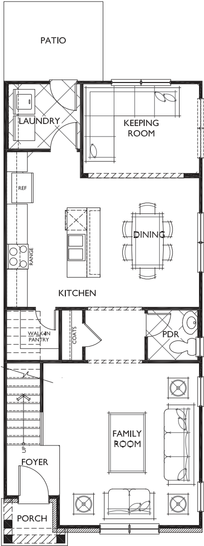
FIRST FLOOR
